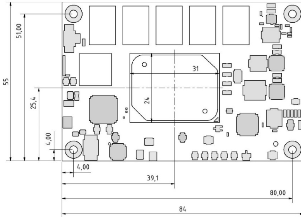
Figure 7: Module Dimensions
